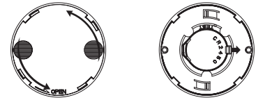
(1) Twist the back cover of smart button and remove it. (2) Pry off and replace with 1x CR2450 battery.
