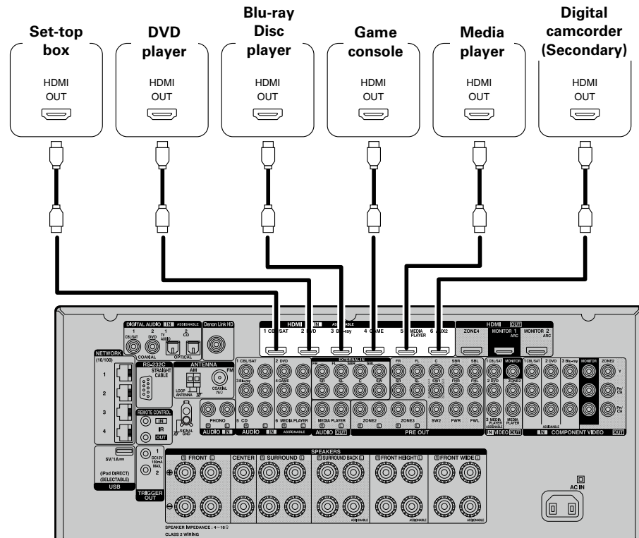
[Rear panel]
